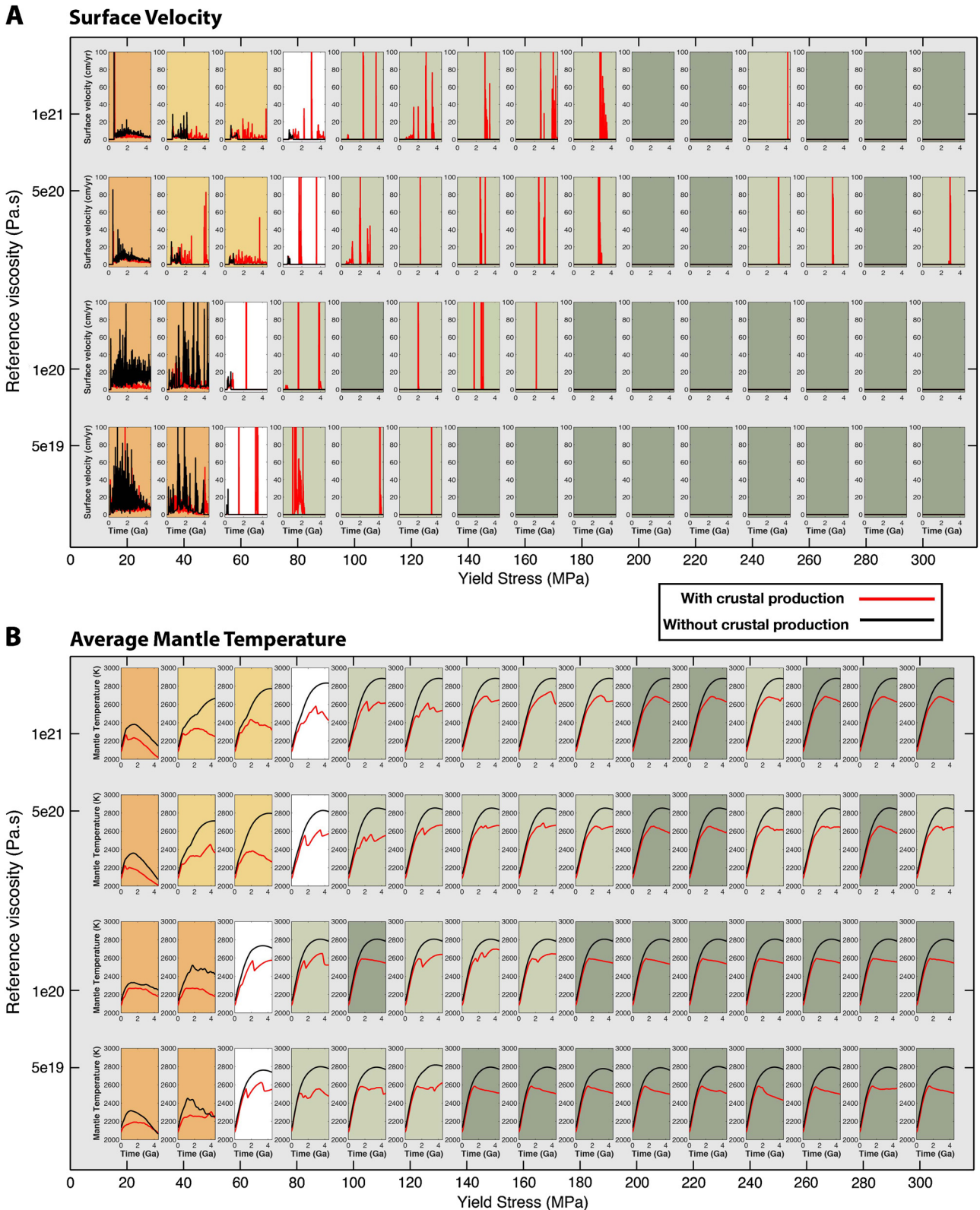
Fig. 3. (A) Surface velocity and (B) average mantle temperature as a function of time for all numerical simulations in the parameter space of yield stress and reference viscosity. For each reference viscosity and yield stress, two cases are represented, one with MCP (red line) and one without MCP (black line). The background colour of each subplot represents the convective regime (or transition between different convective regimes due to MCP): (dark orange): mobile, (light orange): transition from early-mobility to mobile, (white): transition from early-mobility to episodic, (light green): transition from stagnant to episodic, and (dark green): stagnant.
