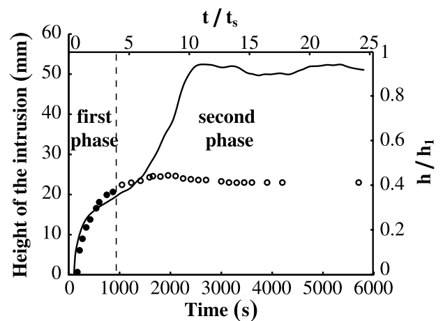
Figure 9. Height of the intrusion in experiment 10 (dots) and simulation 36 (solid line) which are made in almost identical conditions. In a first penetration phase, there is no convection in the upper layer. In the second phase, an active upwelling develops in the upper layer and entrains a thin thread of lower liquid which rapidly rises to shallow levels and almost reaches the top surface (horizontal line at h/h_1 = 1 ). The inflection point on the solid line marks the separation between the two phases. The laboratory technique tracks the top of the bulk intrusion and does not pick up the thin thread. Note the good agreement between the observed and calculated displacement values in the first deformation phase.
