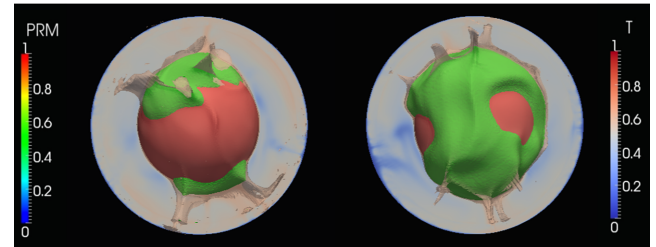
Figure 11. Snapshot of cases with B = 0.30 , \Delta\eta_T = 10^9 , t = 0.0117 (4.5 Gyr) and (from left to right): X_{\text{vol}} = 3.5, 10 per cent. A combination of isosurface of the composition C = 0.5 and non-dimensional temperature T = 0.6 to show the locations of the hot plumes from the dense reservoirs.
