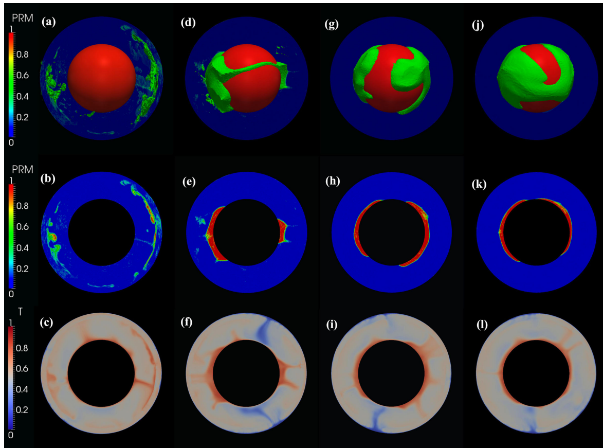
Figure 2. Snapshot of cases with (from left to right): B = 0.16, 0.26, 0.36, 0.50 , \Delta\eta_T = 10^9 , \Delta\eta_C = 1 , X_{\text{vol}} = 3.5 per cent, \Gamma_{660} = -2.5 MPa K ^{-1} . Top row: isosurface of the composition with contour level C = 0.5 . Middle row: polar slices of the composition. Bottom row: polar slices of temperature.
