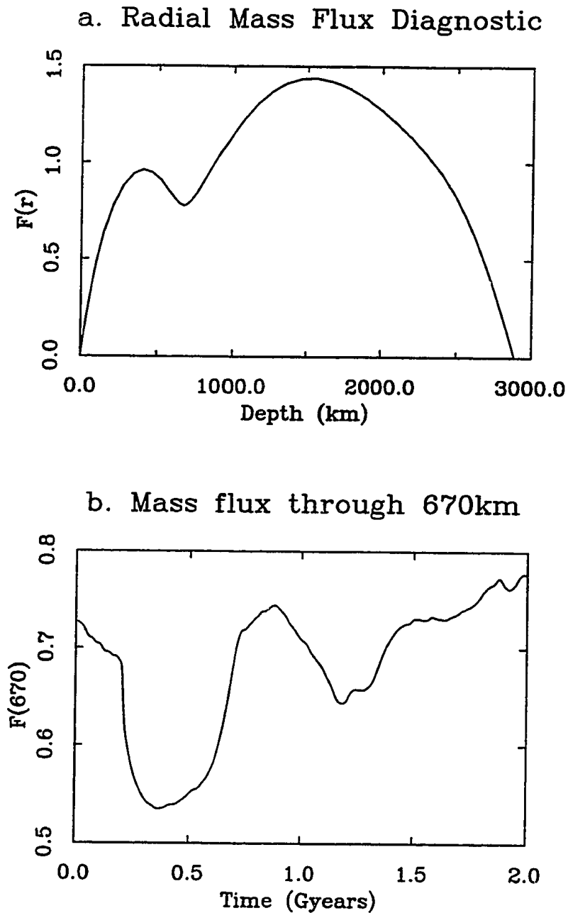
FIG. 2.4 a, Radial mass flux diagnostic F(r) for the final frame of simulation. b, Time series of F(670) for the last 9000 timesteps (2 Gyr). F(r) , defined in Peltier and Solheim , [1992], is the spherically-averaged modulus of radial mass flux, normalized so that the integral over nondimensional depth is unity.
