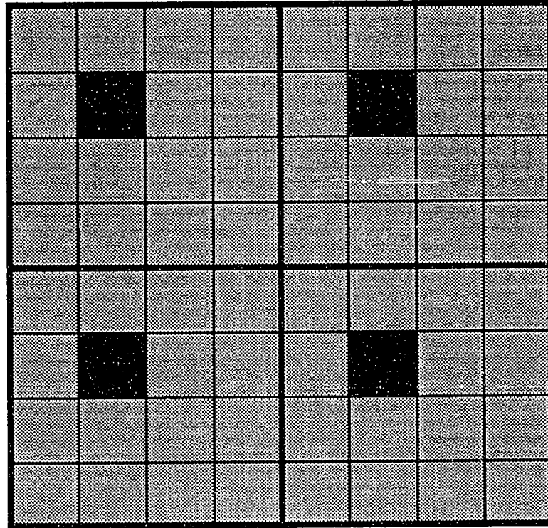
Fig. A.5. Simultaneous decomposition of the FFT and Legendre transforms onto a mesh topology, on 64 nodes. In this case the FFT is decomposed 16 ways, and the Legendre transform 4 ways. FFTs proceed independently in the four 4x4 squares of nodes. Legendre transforms proceed using ring pipelines, with the dark squares indicating one such pipeline.
