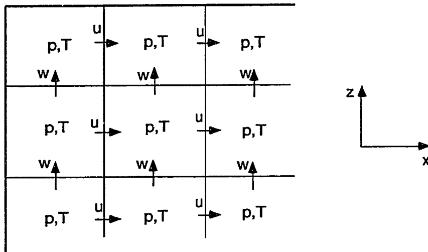
Fig. B.1. A two-dimensional version of the staggered grid. Pressure ( p ) and temperature ( T ) are defined at the cell centers, horizontal velocity ( u ) at the center of the cell walls perpendicular to the x -direction, and vertical velocity ( w ) at the center of the cell walls perpendicular to the z -direction. Vertical and side boundaries (at top and left) coincide with cell walls, allowing easy implementation of boundary conditions.
