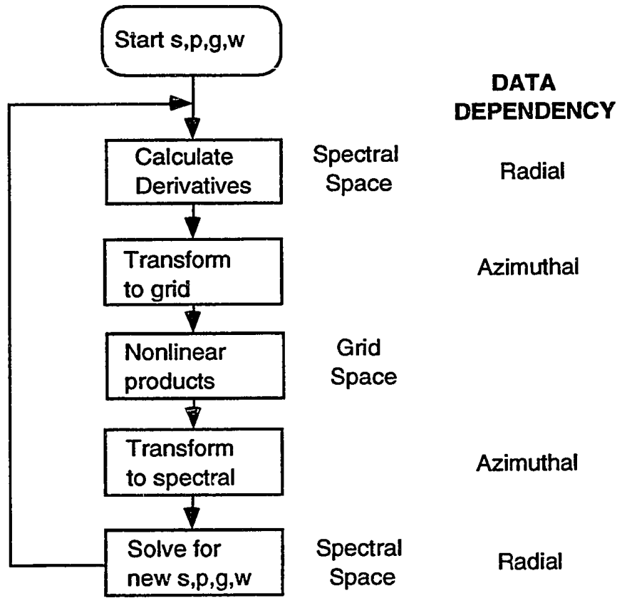
Fig. A.1. Flow diagram showing the various operations involved in one time step.
