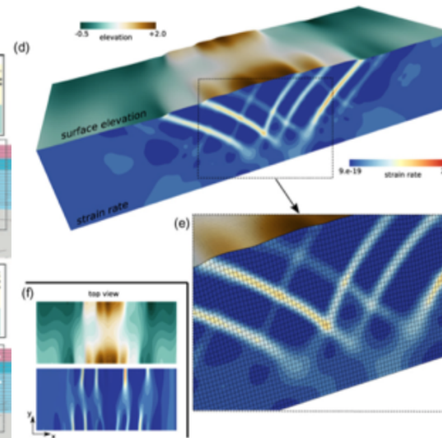
(Thieulot, PEPI, 2011)
